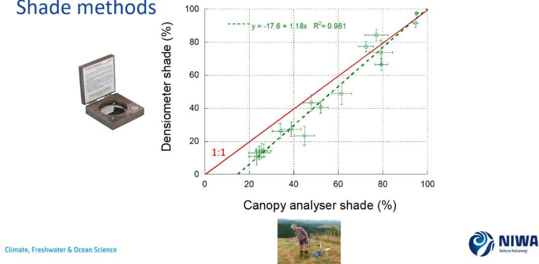
Figure B-1: Relationship between “biased” reach-averaged shade measured with a densiometer and “unbiased” reach-averaged shade measured with a canopy analyser. From Matheson et al. (2018). Measurements made in streams and rivers in the Piako River catchment, Waikato, NZ.
